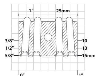
CF-15AP Paslode Type
